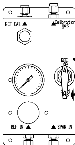
UNIT-C Supply reference gas
