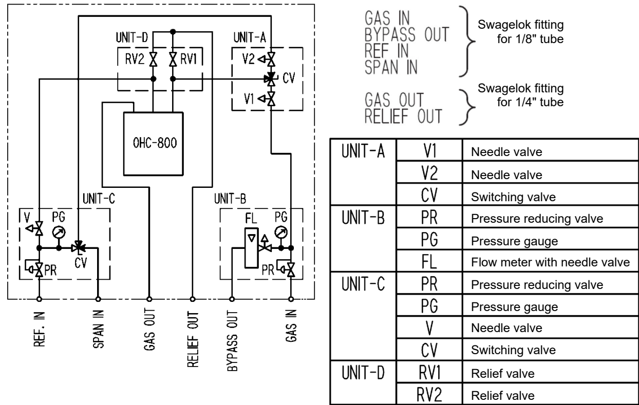
Tubing diagram
