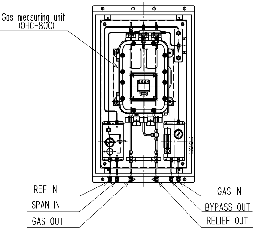
Tubing diagram
