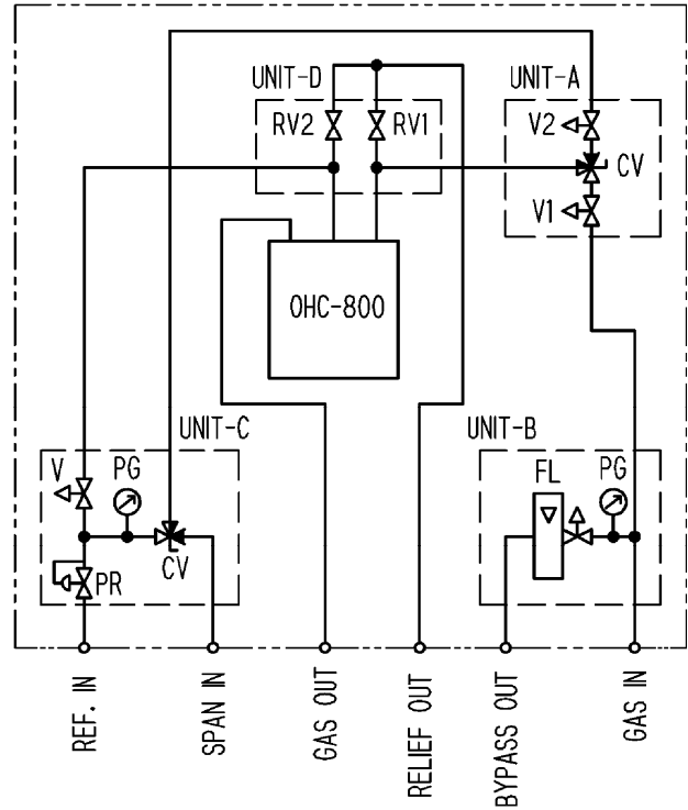
Tubing diagram
