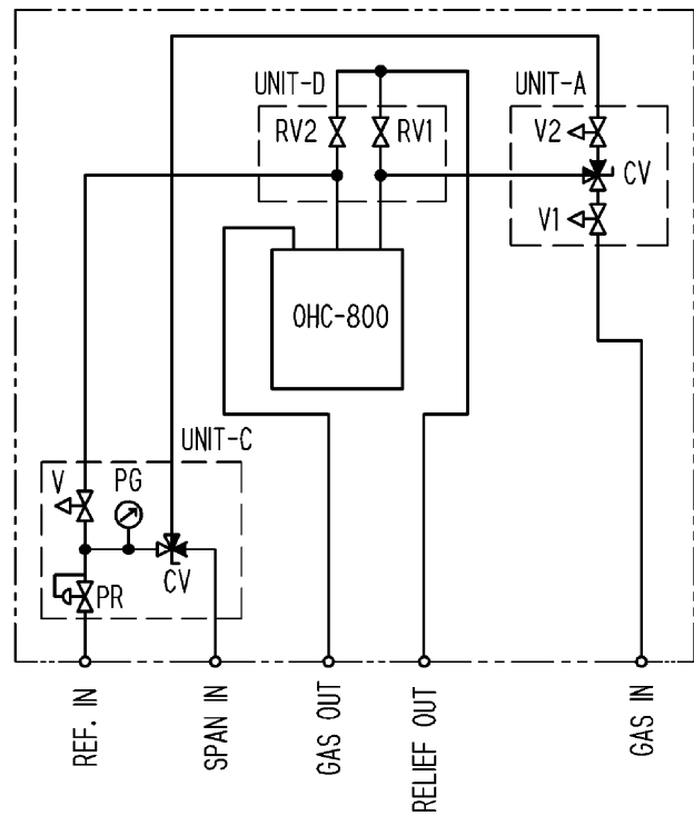
Tubing diagram
