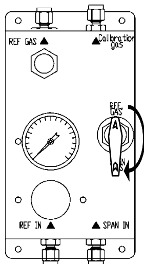
UNIT-C Supply reference gas
