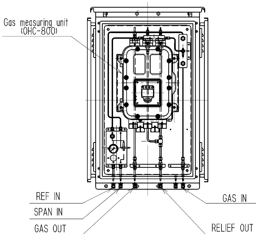
Tubing diagram
