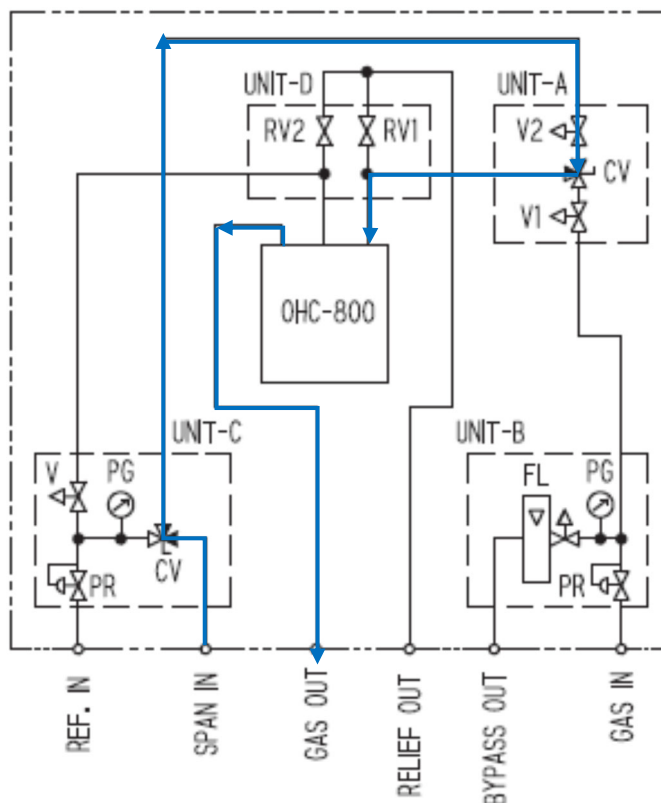
Tubing diagram
