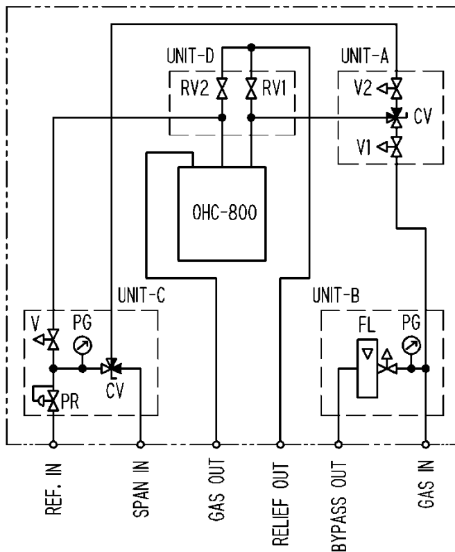
Tubing diagram
