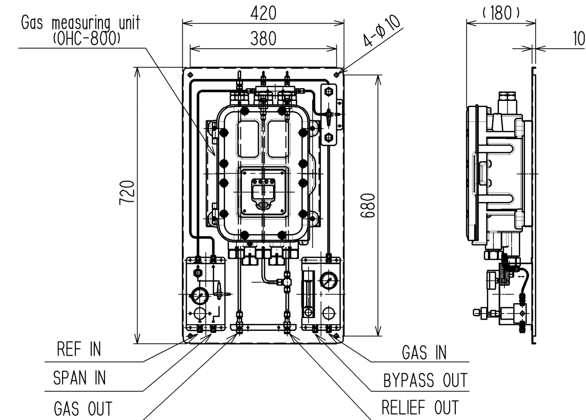
Tubing diagram
