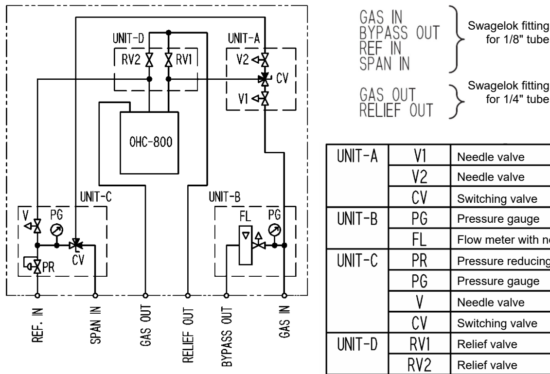
Tubing diagram
