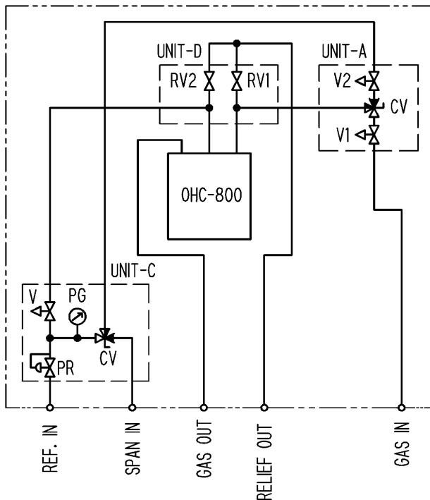
Tubing diagram
