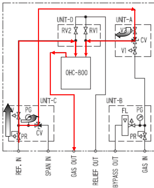
Tubing diagram
