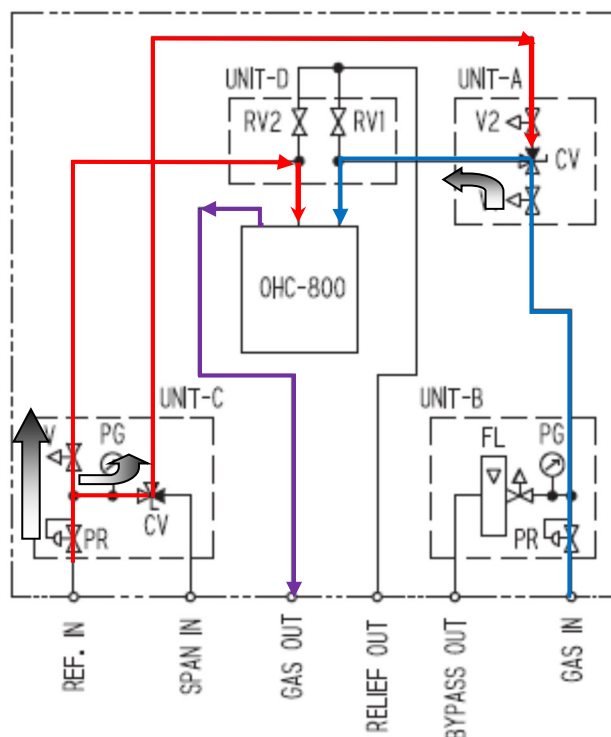
Tubing diagram
