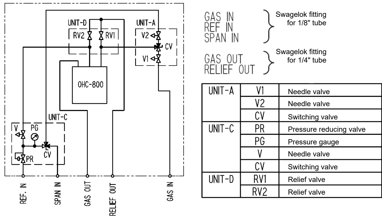
Tubing diagram
