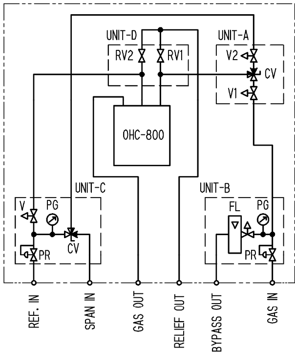
Tubing diagram
