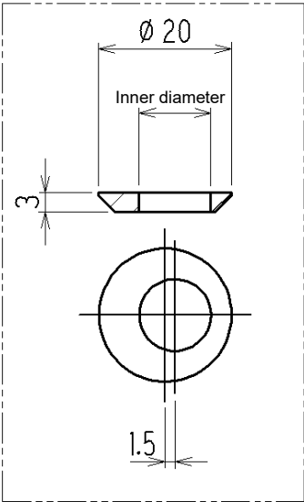
Clamp washer
