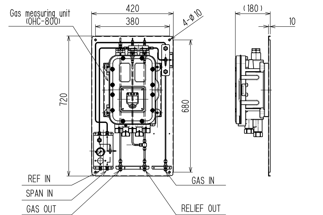
Tubing diagram
