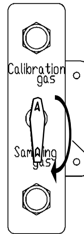
UNIT-A Supply calibration (reference) gas
