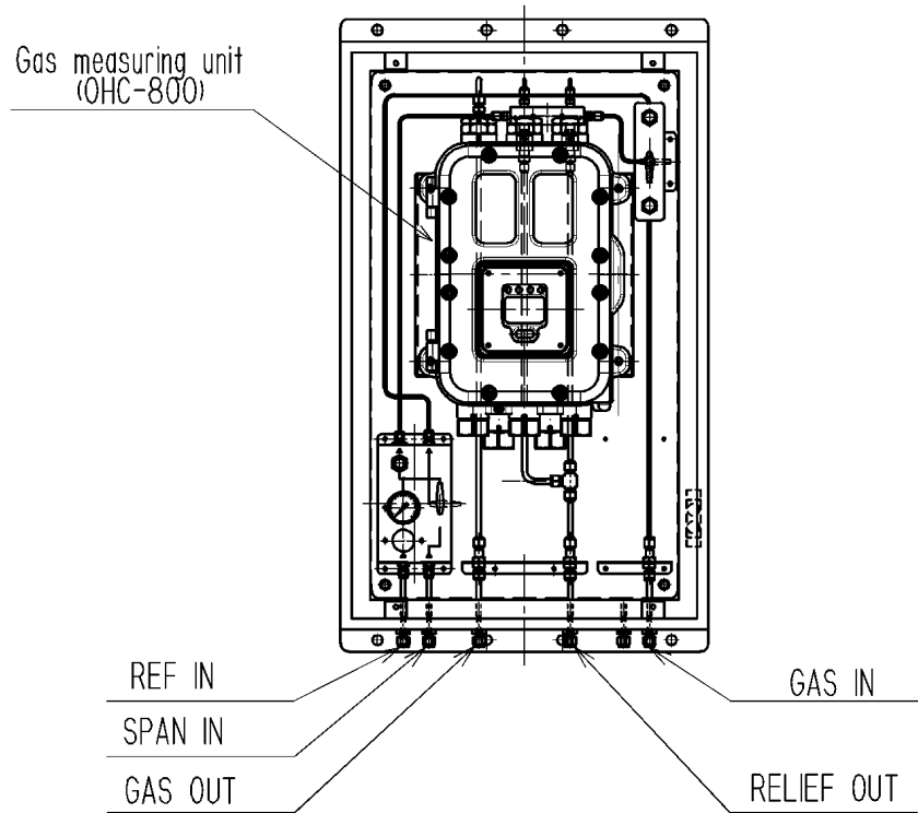
Tubing diagram
