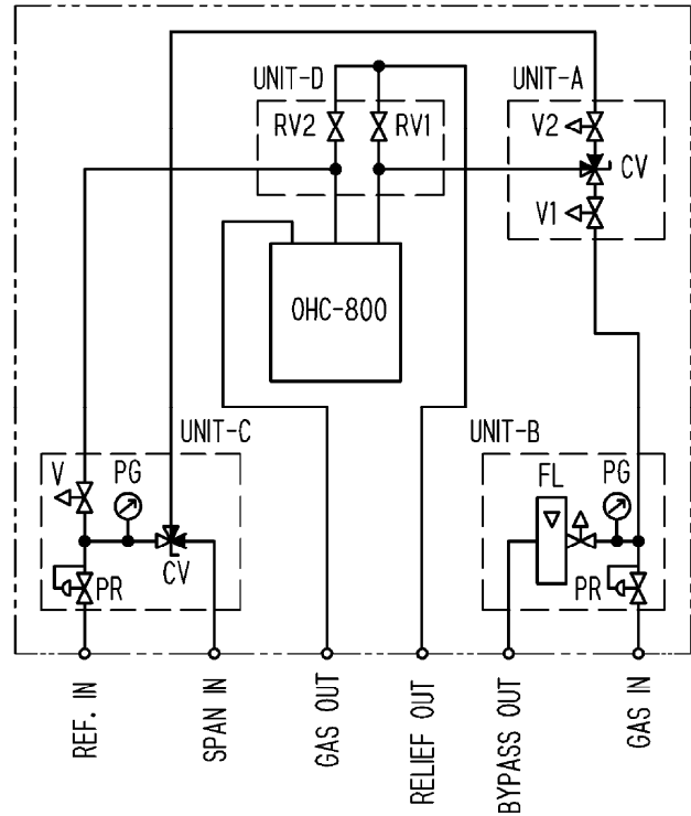
Tubing diagram
