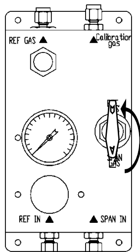
UNIT-C Supply reference gas
